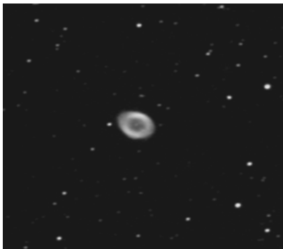
M57 - Lyra
