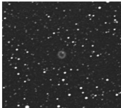
NGC6894 - Cygnus
